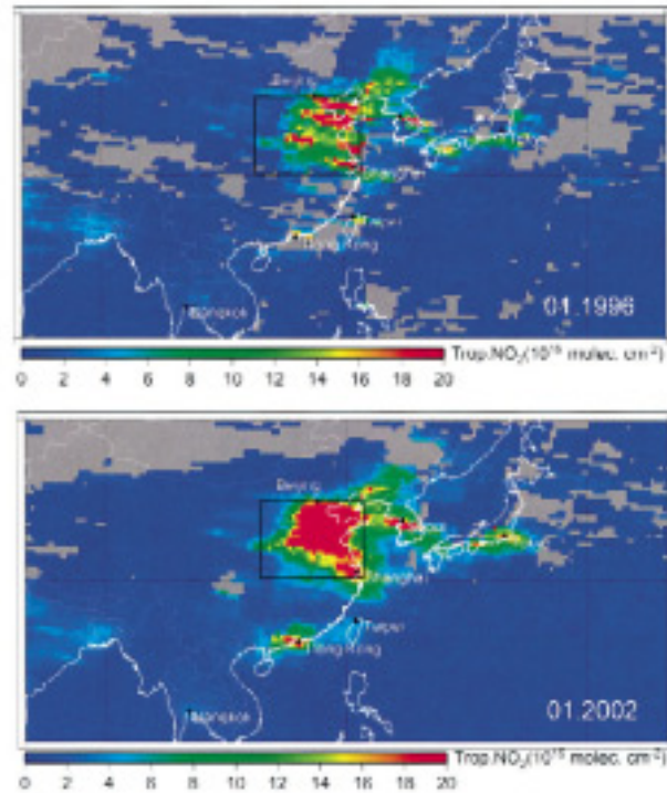
Figure 2-1. Distribution of NO 2 concentrations in the troposphere of East Asia, measured by the Global Ozone Monitoring Experiment. Shown here are average January concentrations in 1996 (top) and 2002 (bottom). Gray zones indicate lack of data. (JAMSTEC 2005)
