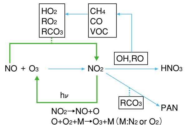
Figure 1-6. Generation and transformation process of ozone and nitrogen compounds.
