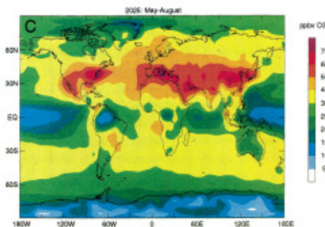
Figure 1-3. Modeling prediction on geographical distribution of ground-level ozone concentrations in 2025 (average from May to August). (Lelieveld and Dentener 2000)
